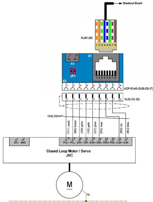
An EdingCNC / Simple BOB
