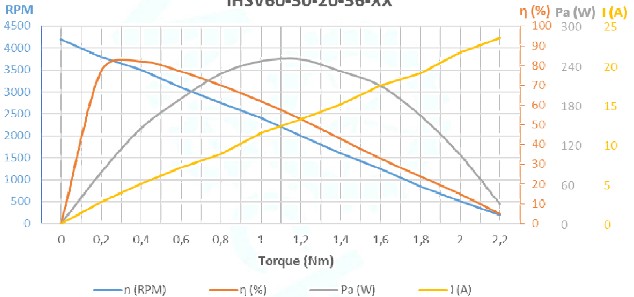
Power curve iHSV60-30-20-36-XX
