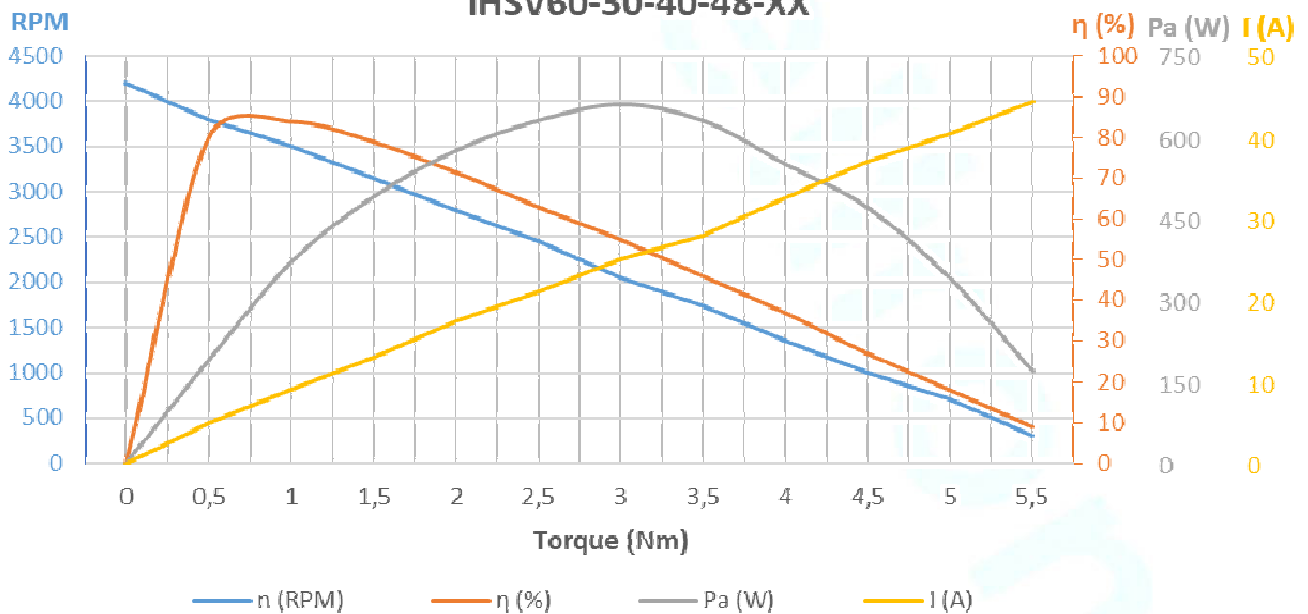
Power curve iHSV60-30-40-48-XX
