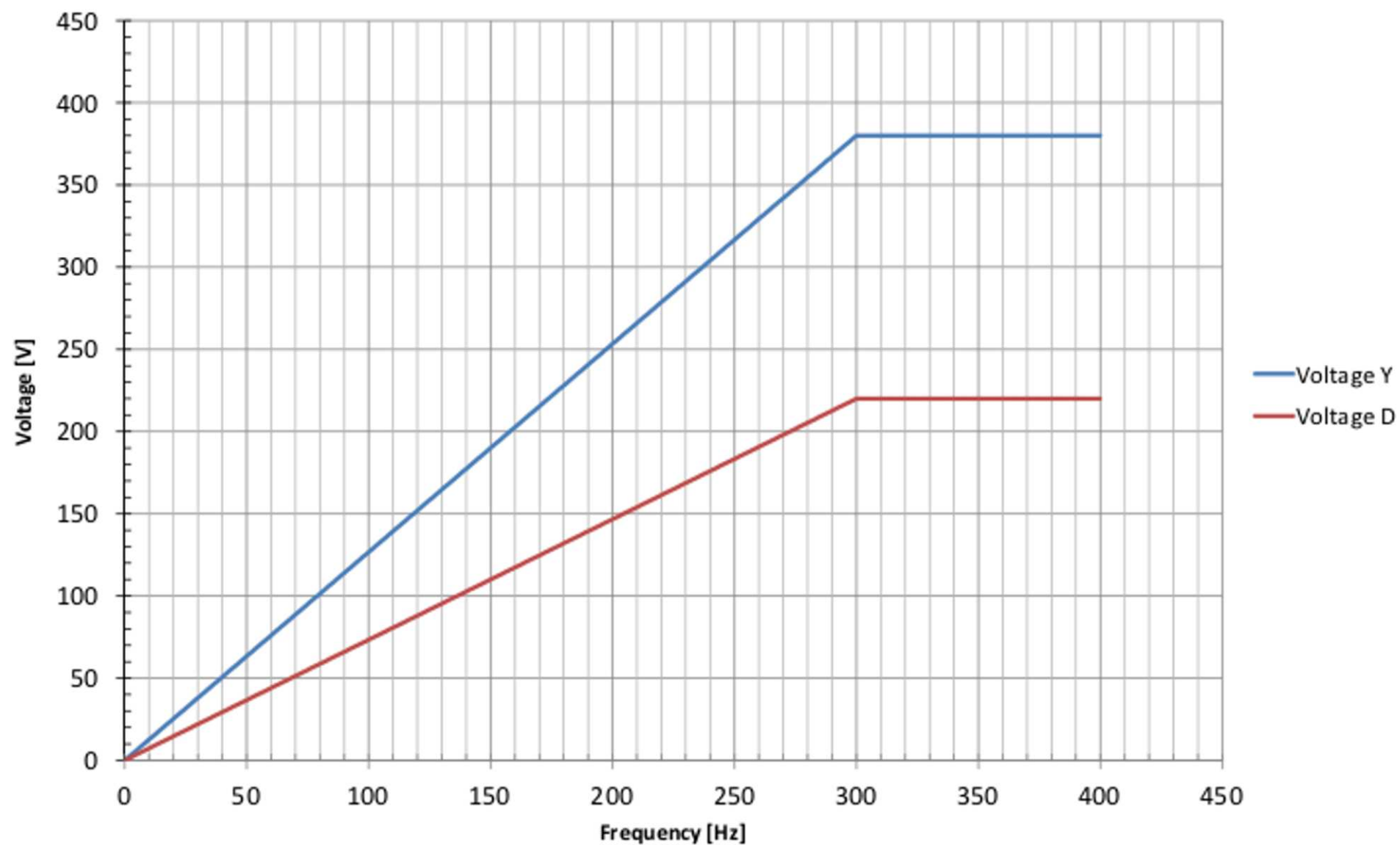
COM31400414 - Voltage-Frequency curve for inverter programming
