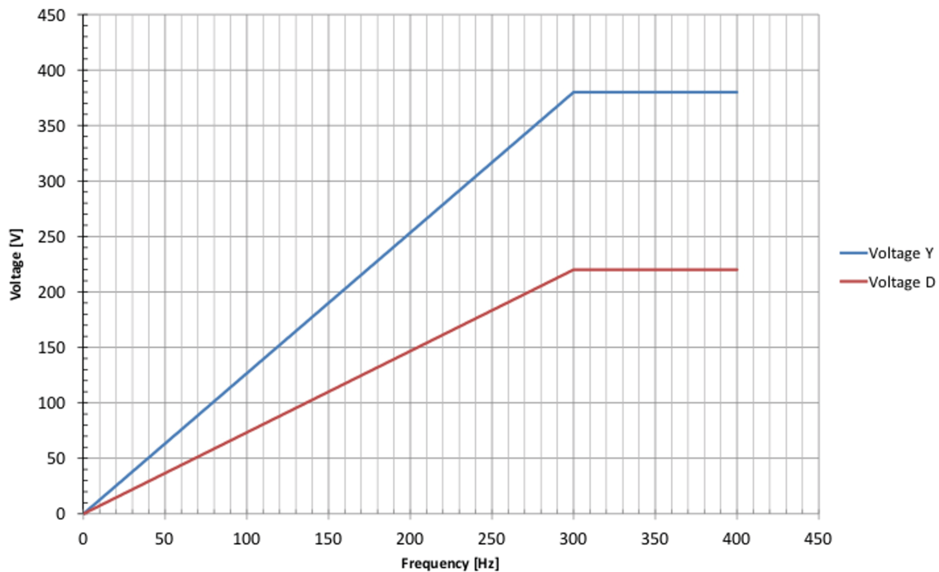
COM31400404 - Voltage-Frequency curve for inverter programming
