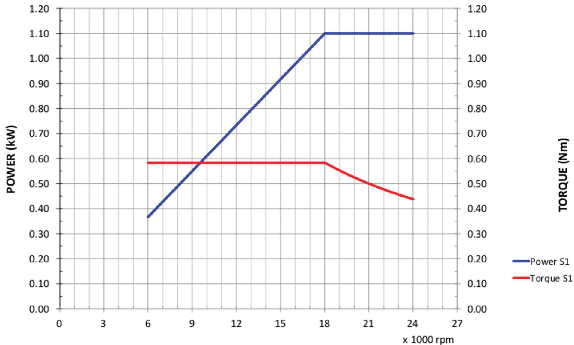
COM31400404 - POWER-TORQUE CURVES
